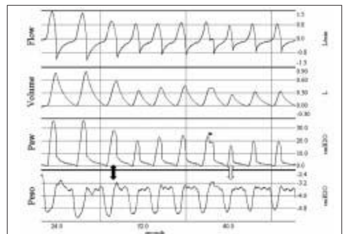
Figure 4: Example of proportional assist ventilation with a high degree of gain (90% of flow and volume assistance). Airway pressure (Paw) grossly follows esophageal pressure (Peso). Large Peso swings produce bigger pressure assistance (full arrow) and vice versa (empty arrow). This example was obtained with a Puritan Bennett 840 (Tyco Healthcare, Mansfield, MA). This ventilator automatically performs tele-inspiratory pauses during PAV to measure elastance (*)
