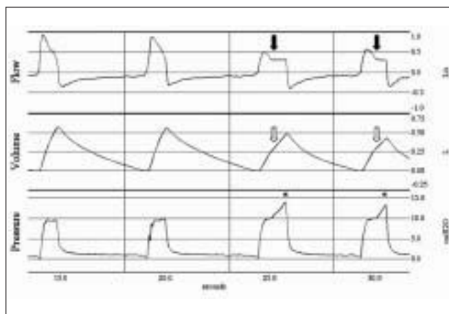
Figure 2: Ventilation with volume-assured pressure support (VAPS). The first two inspirations are pressure-targeted cycles. During the next two inspirations, delivered volumes are less than the desired minimum tidal volume (empty arrows) when instant inspiratory flow reaches the “constant flow level” (full arrows). At this point, the ventilator delivers a constant inspiratory flow to attain the minimum tidal volume. Thus, an increase in airway pressure is observed (*)
