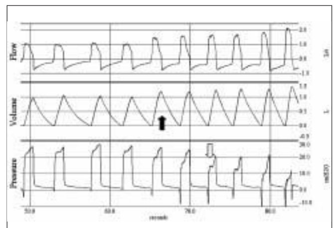
Figure 3: Example of adaptive pressure ventilation (APV). In this case, tidal volume increases due to a larger patient’s demand (full arrow). APV inappropriately reduces pressure level during the next cycles (empty arrows). This type of response can also be seen during volume support (VS)
